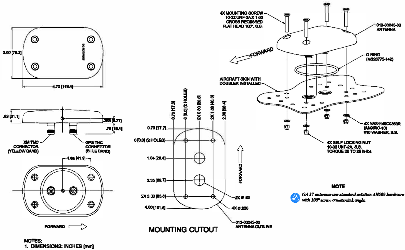
Figure A-3. GA 37 Antenna Installation Drawing
